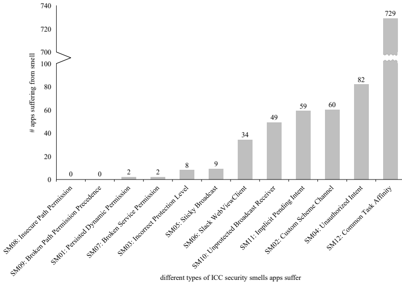
Figure 5.1: Distribution of security smells in the apps
