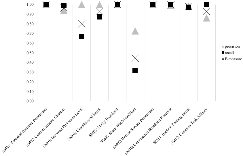
Figure 5.9: Tool performance
