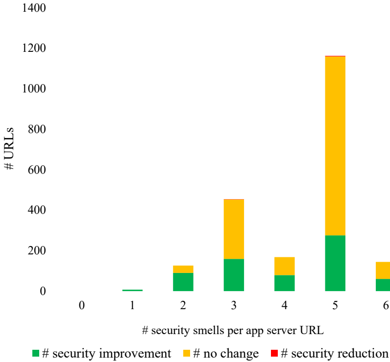
Figure 7.12: Correlation between app server security smells and configuration changes
