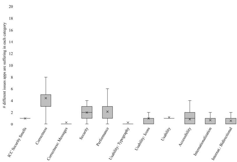
(a) 100 least vulnerable apps
