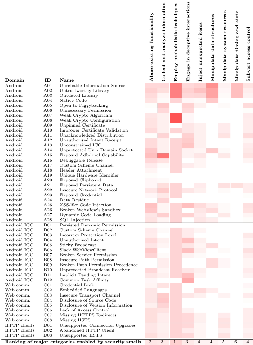
Figure 9.1: Security smells categorized by the CAPEC taxonomy
