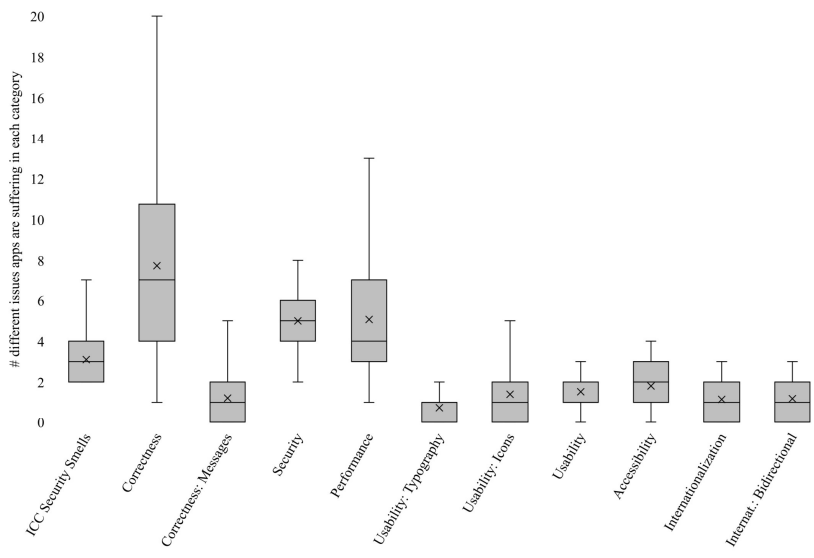
(b) 100 most vulnerable apps
