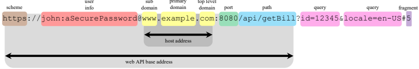
Figure 2.2: The structure of a URL
