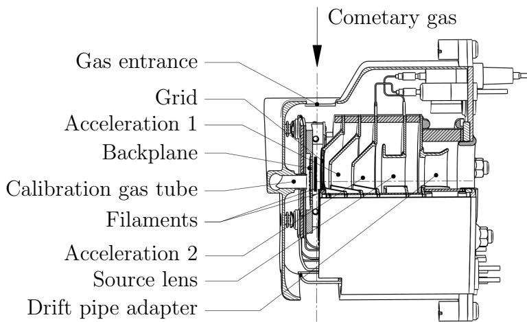
Figure 2.2: Sectional view of the Storage Source.
