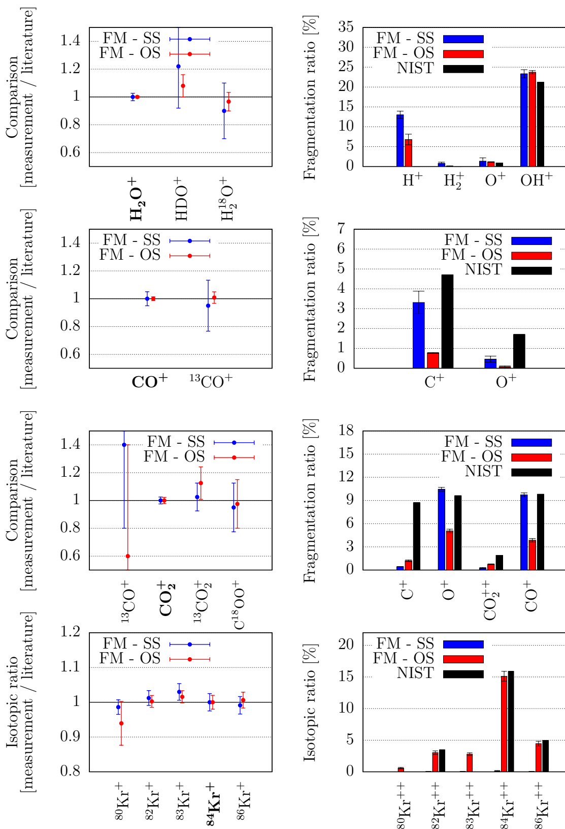
Figure 4.22: H 2 O, CO, CO 2 , and Kr ratios. For H 2 O, CO, and CO 2 , on the left side, the points correspond to the isotopolog ratios measured with RTOF divided by the ones from literature (NIST); on the right side, fragmentation ratios are given relative to the parent. For Kr, singly charged isotopes are shown on the left panel and are relative to the literature (NIST), doubly charged ions are shown on the right panel and are relative to the main isotope ( 84 Kr + ). When not specified, C = 12 C and O = 16 O.
