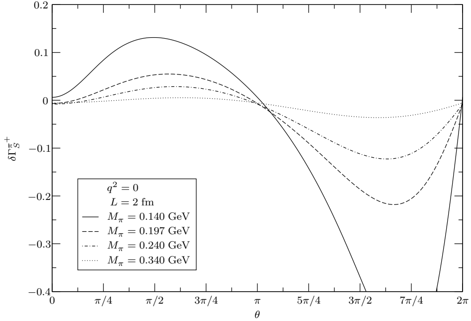
(b) Angle dependence of \delta\Gamma_S^{\pi^+} at q^2 = 0 .
