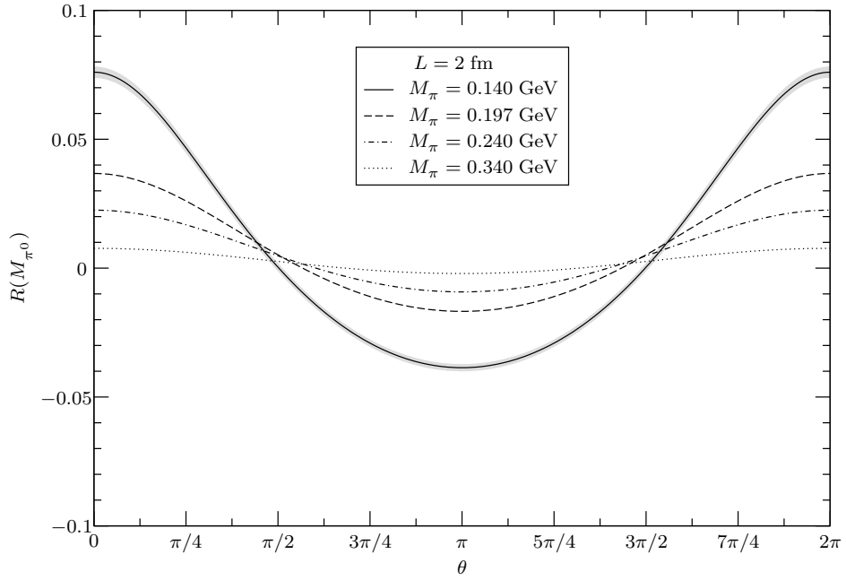
Figure 5.20: Mass corrections of the neutral pion beyond NLO.
