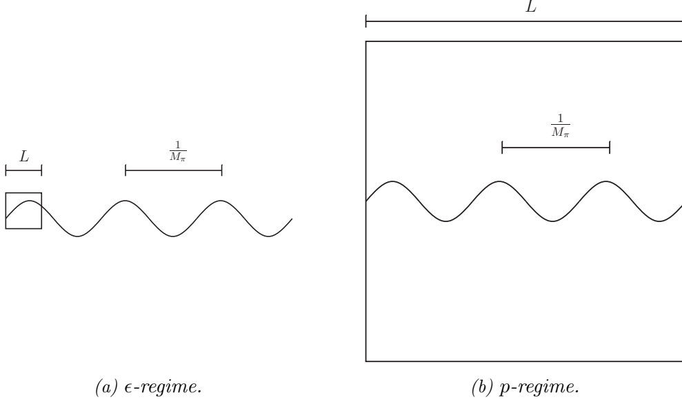
Figure 2.1: Propagation of pions in finite volume. In the \epsilon -regime (a) the Compton wavelength of pions is larger than the side length L and pions can not properly propagate within the volume. In the p -regime (b) the Compton wavelength is smaller than L and pions propagate within the volume in a periodic way.
