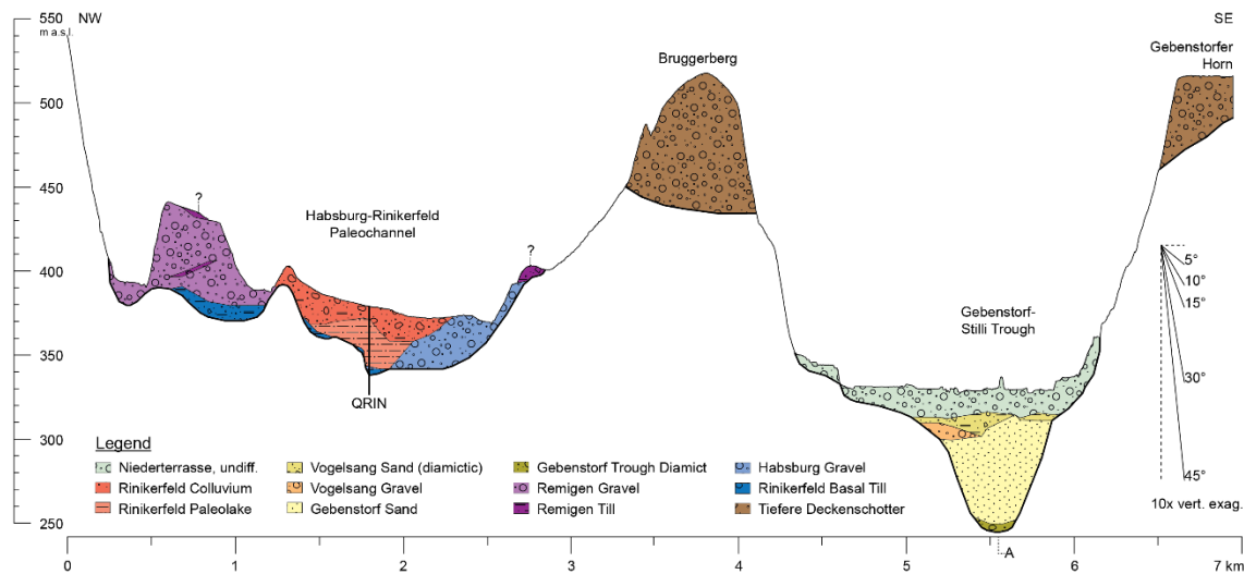
Fig. IV-10: Cross-section B (see Fig. IV-1 for location) through the study area illustrating the stratigraphy of the HRPC and the overdeepened GST. A: Intersection with profile A (Fig. IV-9).
