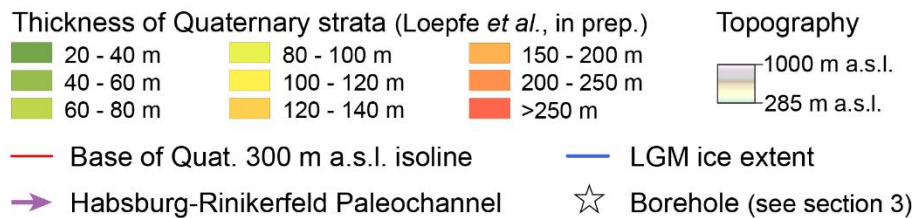
Fig. I-7: Overview map of the Wasserschloss area with major Pleistocene landforms (see Fig. I-6 for localisation).
