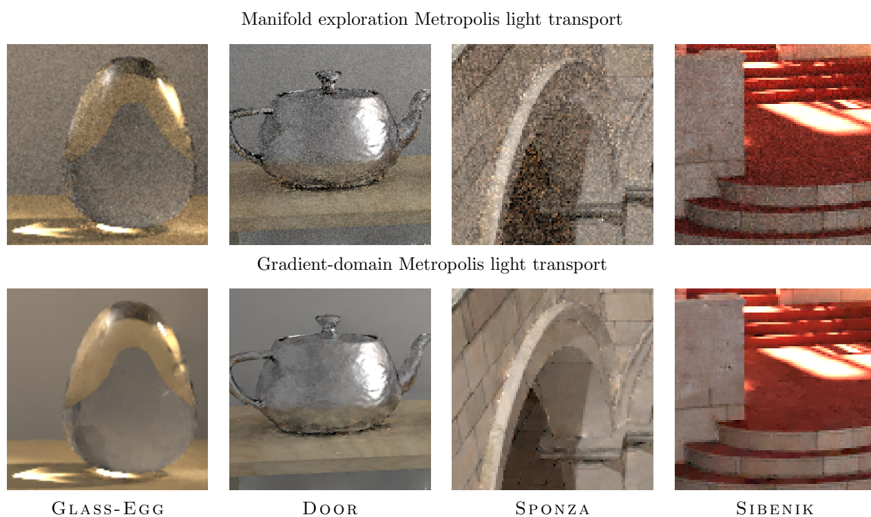
Figure 5.13: Comparison of MEMLT [45] to G-MLT [68] in different scenes. The top and bottom images used roughly equal time to render.
